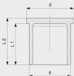
Čep - bakar Model 95290
