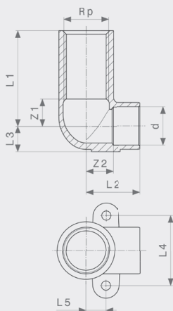
Zidna pločica - bronca Model 94472GL
