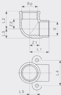
Zidna pločica - bronca Model 94472G
