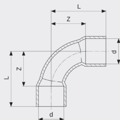
Luk 90° - bakar Model 95002A
