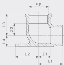
Zidna pločica - bronca Model 94471G
