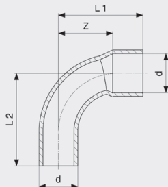
Luk 90° - bakar Model 95001A
