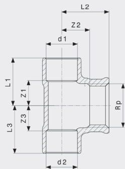
T-komad - bronca Model 94130G
