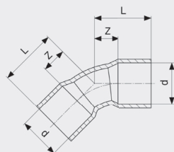
Luk 45° - bakar Model 95041
