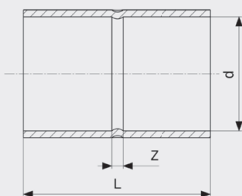
Spojnica - bakar Model 95270
